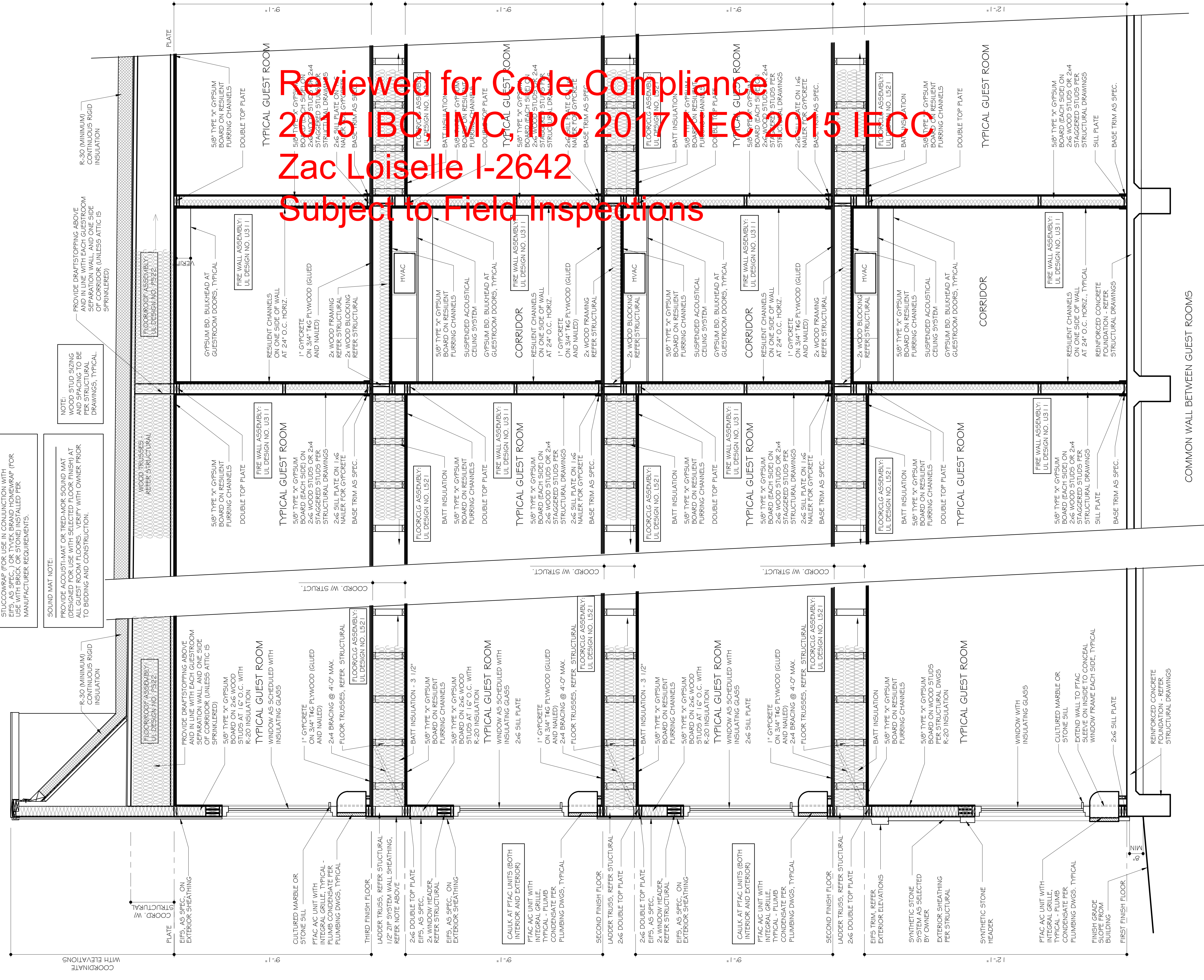
1 BUILDING SECTION SCALE: 1/2" = 1'-0"
